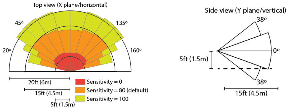
Figure 3: PIR Sensitivity
